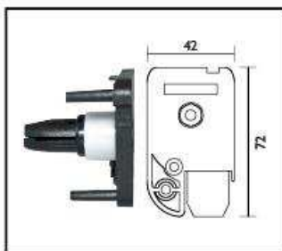
KIT P42
